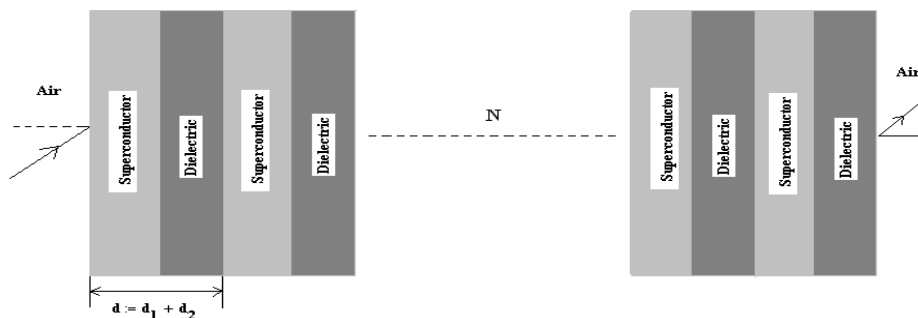
Figure 1. Schematic presentation of superconductor/dielectric periodic structure.
