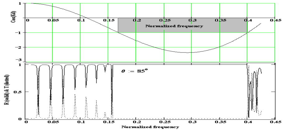
Figure 2: Dispersion relation, Reflectance and Transmittance of the considered structure at an angle of incidence (a) 0^\circ (b) 30^\circ (c) 60^\circ and (d) 85^\circ .
