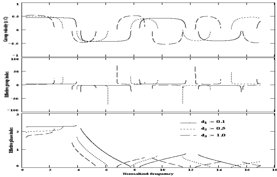
Fig (2): Group velocity, Effective group index and effective phase index Vs Normalized frequency at plasma frequency = (5.6 \times 10^{11}) \times 1 , N=15 and n = 2.35 (ZnS).
