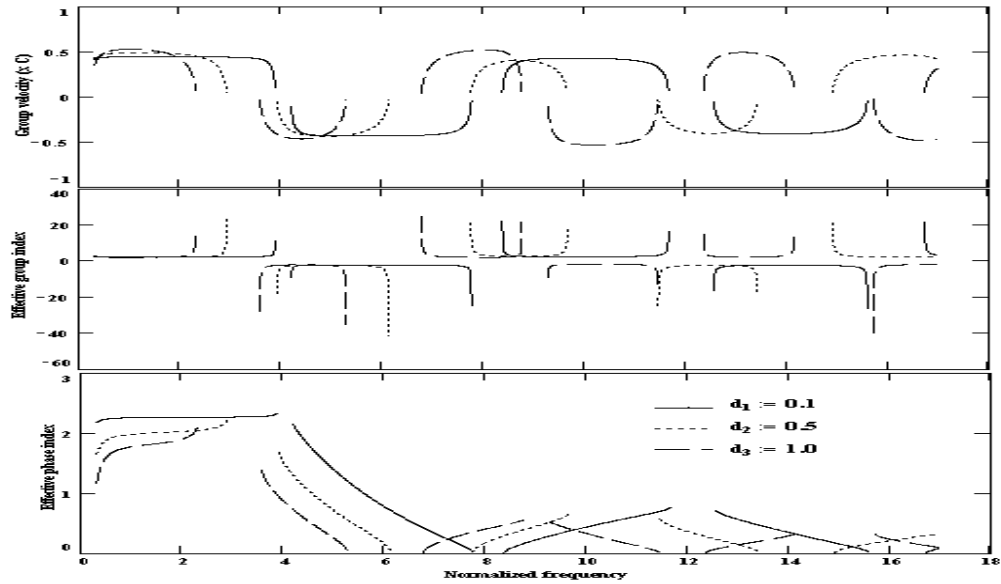
Fig (4): Group velocity, Effective group index and effective phase index Vs Normalized frequency at plasma frequency = (5.6 \times 10^{11}) \times 2 , N=15 and n = 2.35 (ZnS).
