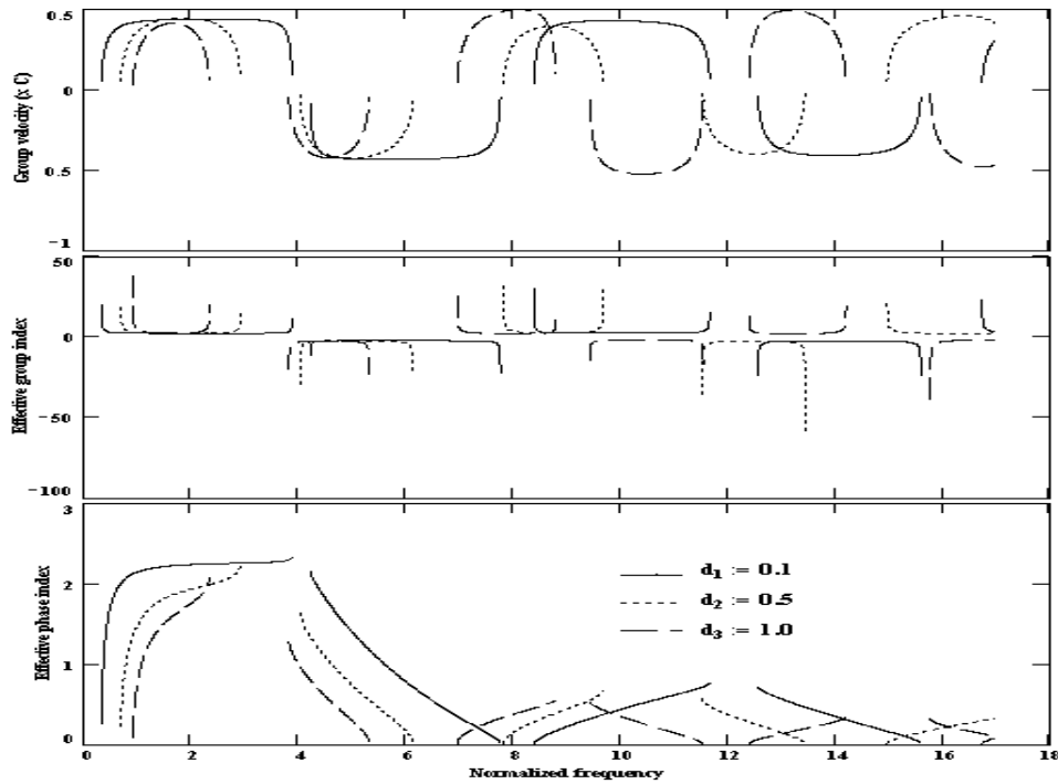
Fig (6): Group velocity, Effective group index and effective phase index Vs Normalized frequency at plasma frequency = (5.6 \times 10^{11}) \times 8 , N=15 and n = 2.35 (ZnS).
